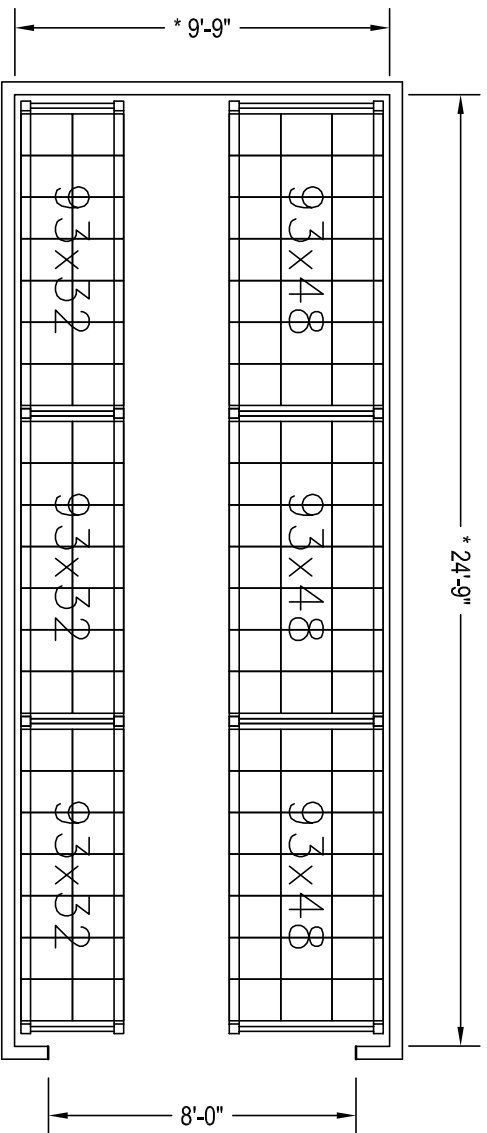
PLAN VIEW
