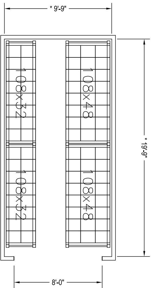
PLAN VIEW
